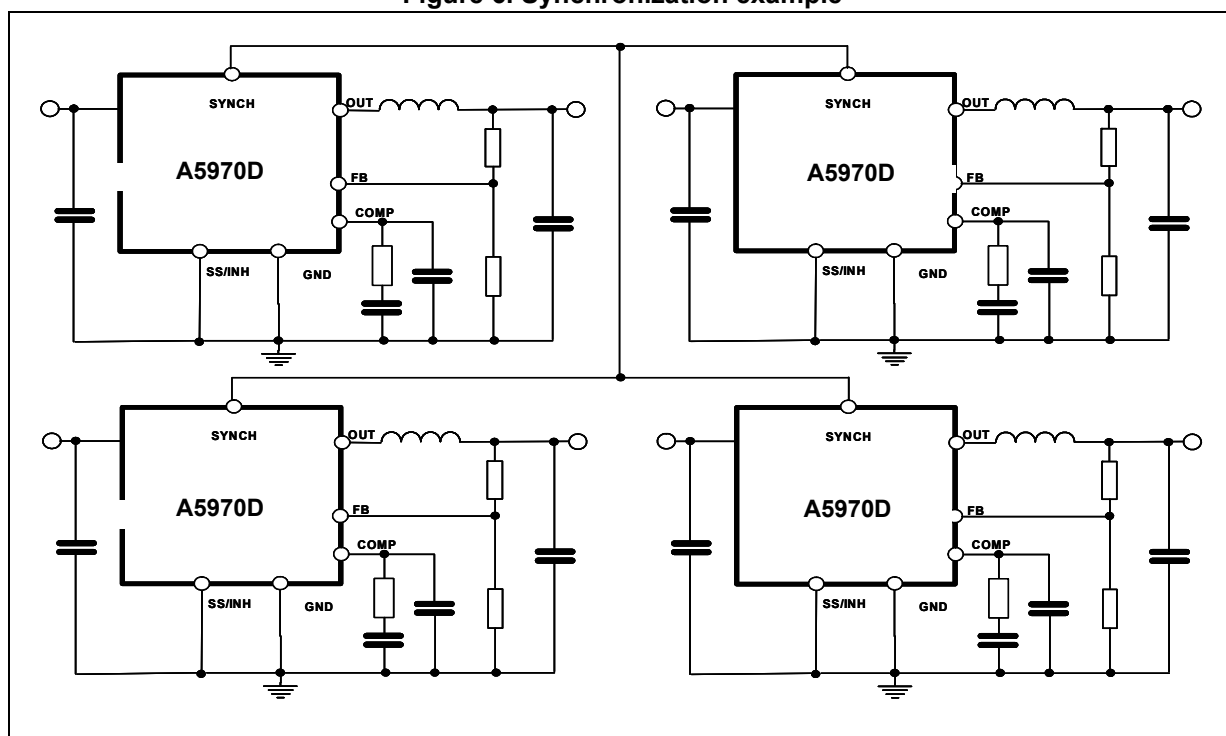
Figure 6. Synchronization example
