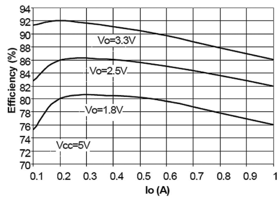
Figure 35. Efficiency vs. output current - V_{IN} = 5\text{ V}
