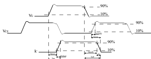
Figure 18. Switching waveform
