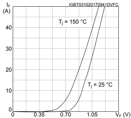
Figure 14. Converter diode forward characteristics (terminal)
