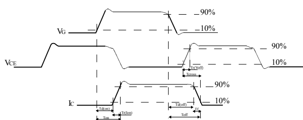
Figure 18. Switching waveform
