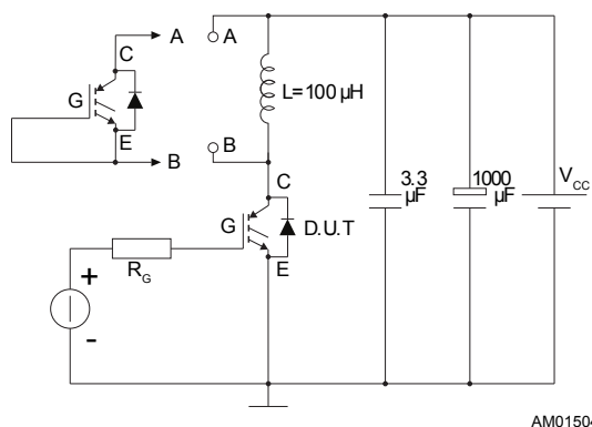
Figure 16. Test circuit for inductive load switching
