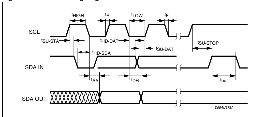
Figure 5. I 2 C bus timing diagram
