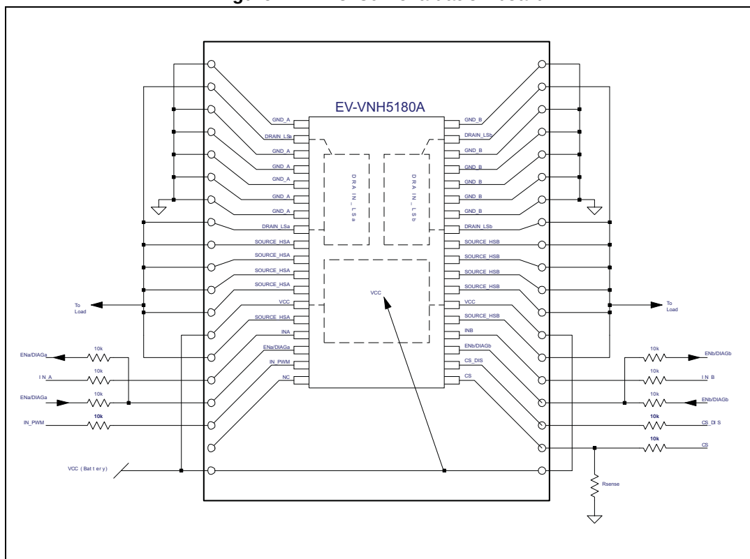
Figure 1. VNH5180A evaluation board
