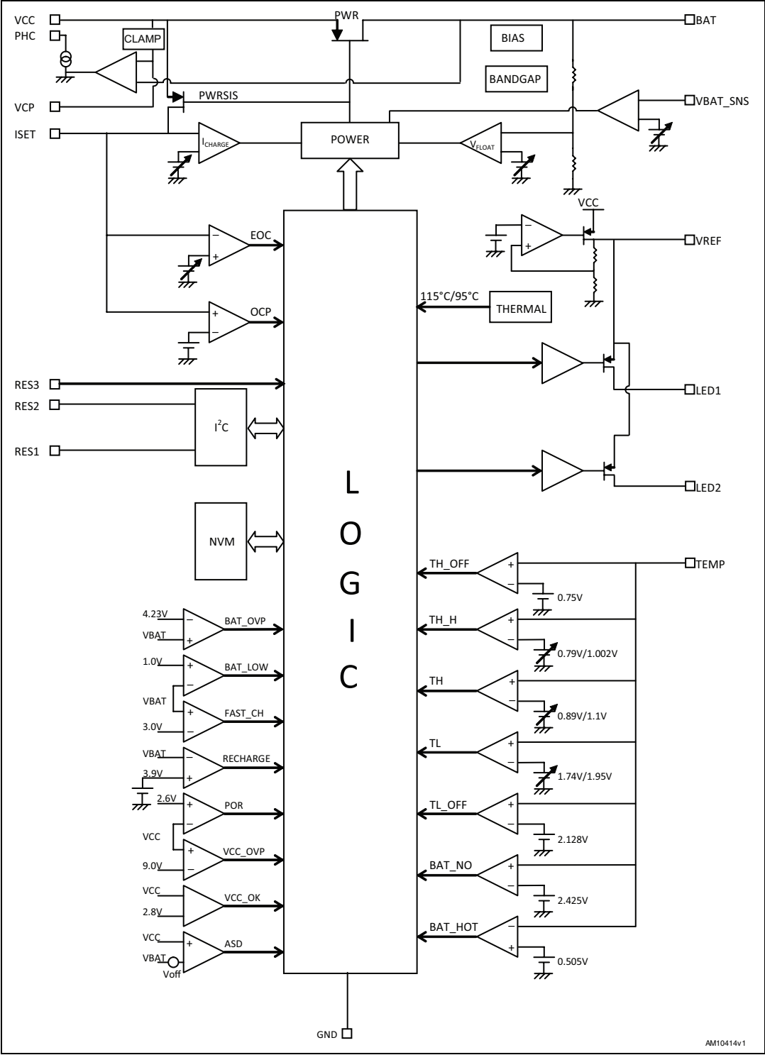
Figure 1. Block diagram
