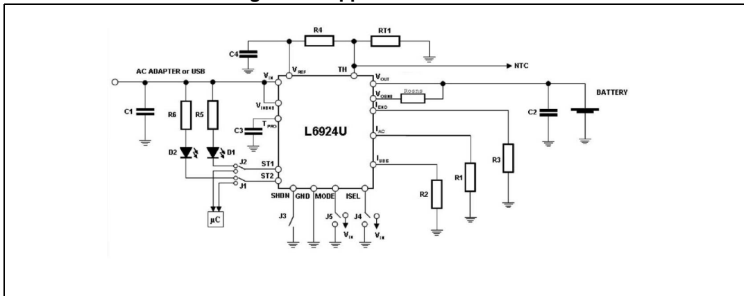
Figure 22. Application schematic
