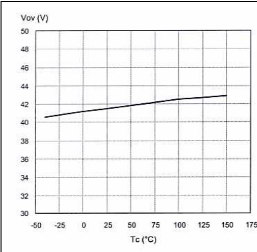
Figure 17. Overvoltage shutdown
