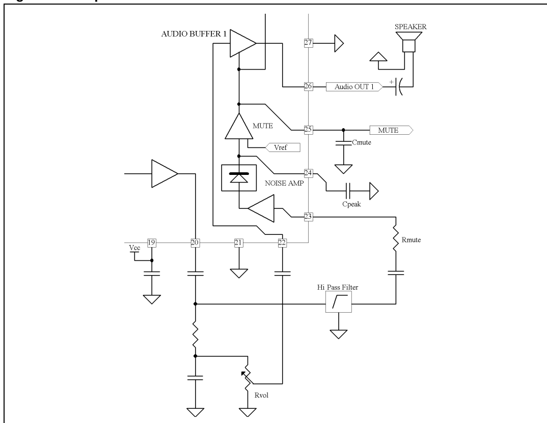
Figure 29. Squelch schematics
