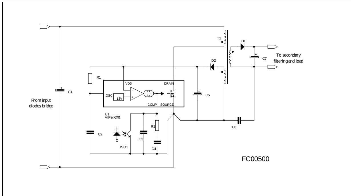
Figure 26. Recommended Layout
