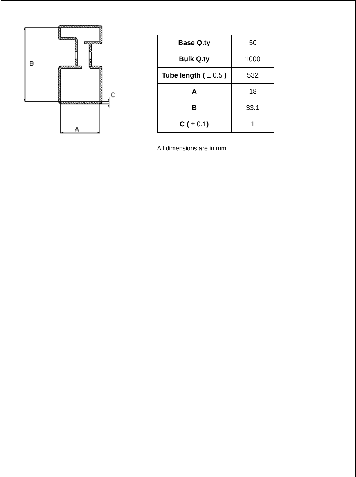
Figure 27. Pentawatt HV Tube Shipment ( no suffix )
