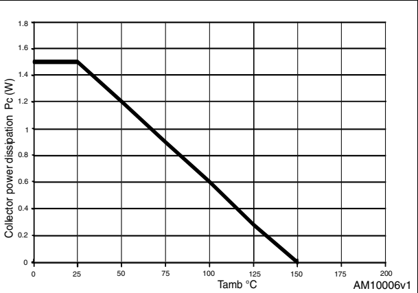
Figure 3. Derating curve
