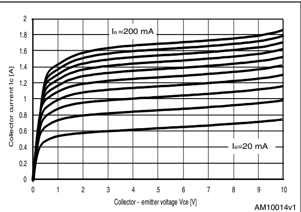
Figure 5. Output curves up to V_{CE}=10\text{ V}
