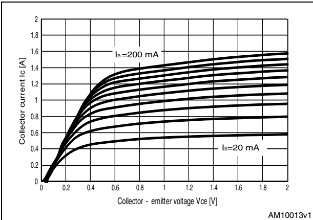
Figure 4. Output curves up to V_{CE}=2\text{ V}
