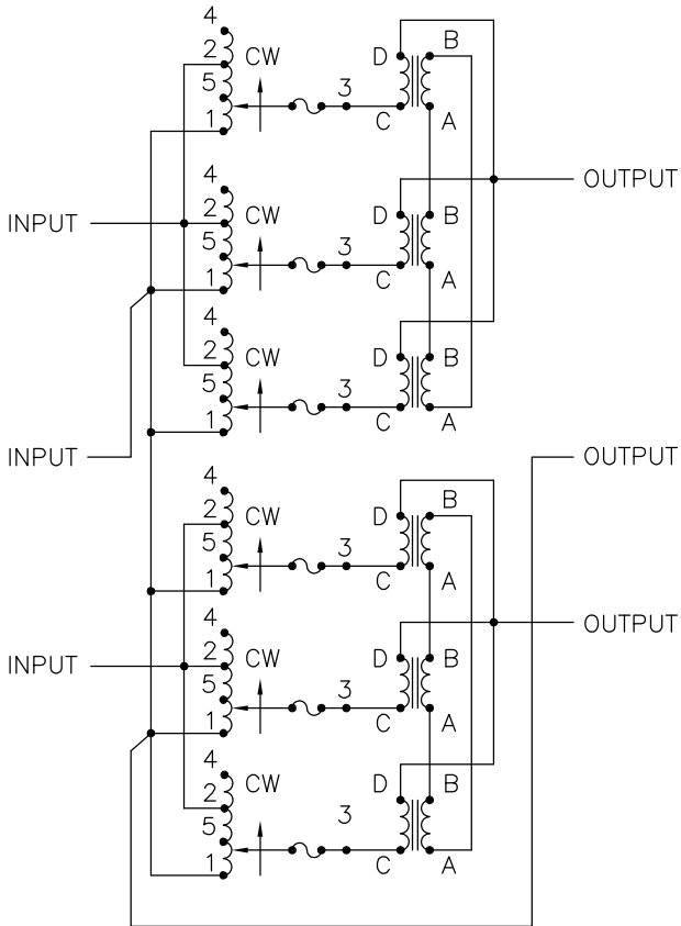
SCHEMATIC
