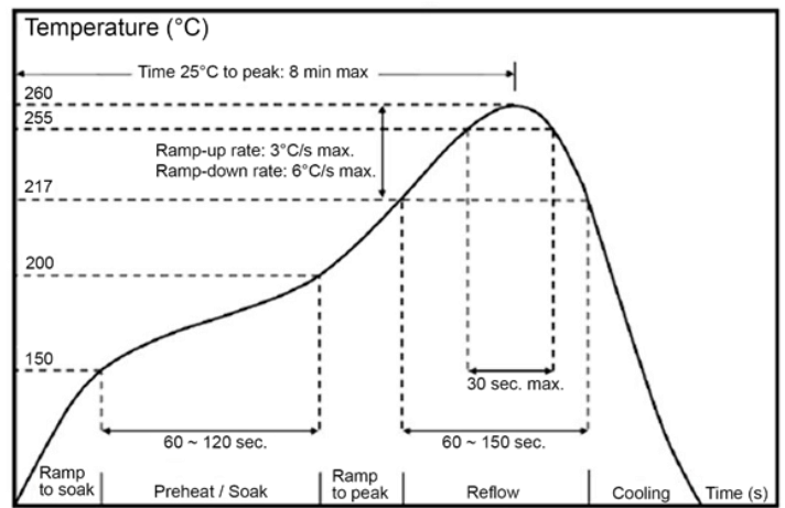
Solder Reflow Temperature Condition
