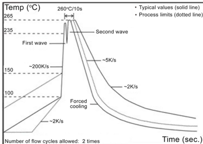
Wave Solder Temperature Condition
