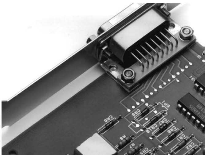
D-Subminiature Connectors
