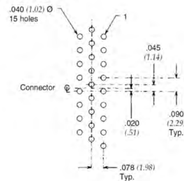
26 High-Density Pin/PCB
