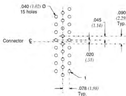
62 High-Density Pin/PCB
