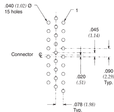
26 High-Density Pin/PCB
