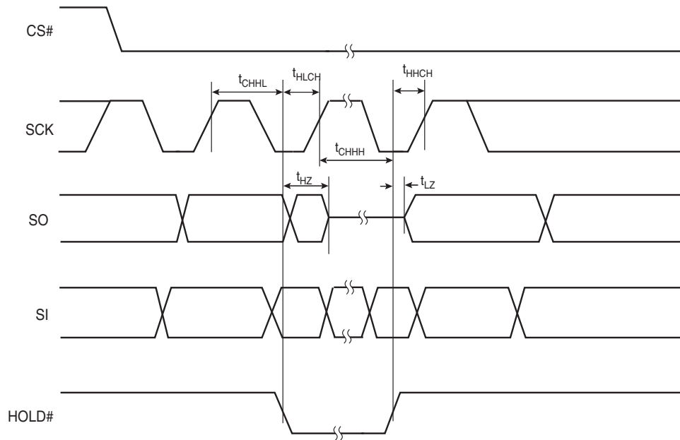
Figure 18.4 HOLD# Timing
