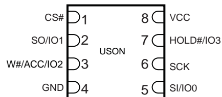
Figure 2.3 8-contact USON (5 x 6 mm) Package
