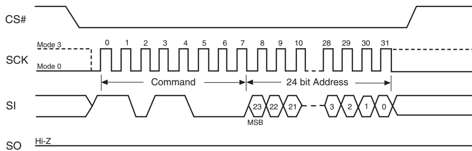
Figure 9.20 Sector Erase (SE) Command Sequence
