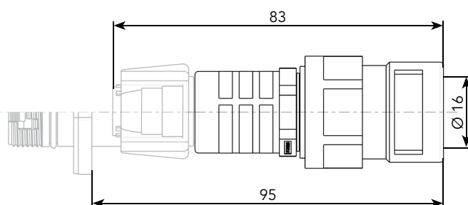
Backshell - WME20008A
