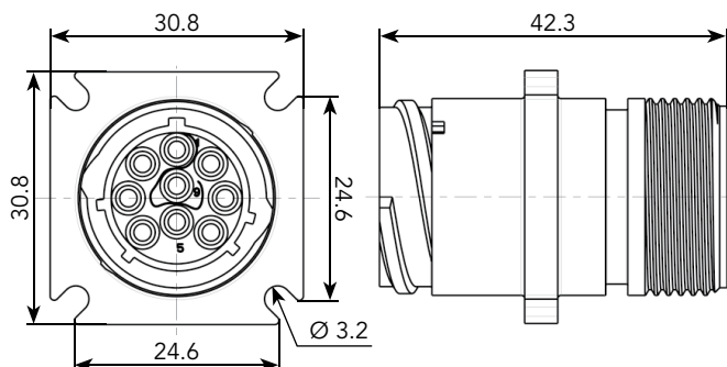
Square flange receptacle - WME20003A/6A
