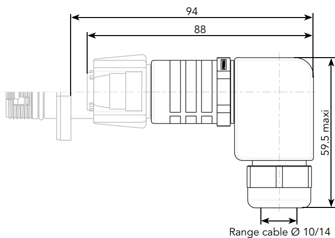
Backshell - WME20010A
