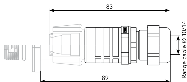
Backshell - WME20009A
