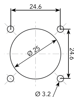
Panel Cut Out
