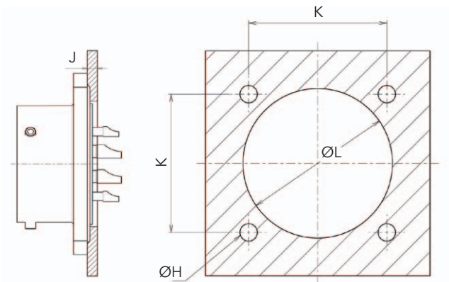
Panel cut-out
