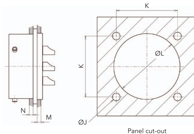
Panel cut-out
