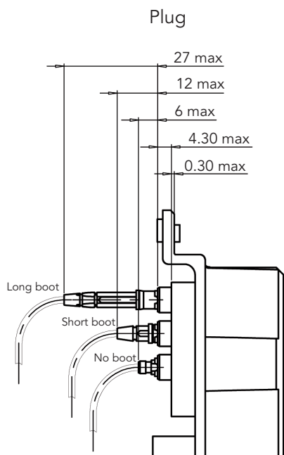
ELIO® contacts in ELIO® AQ adaptor for #8 cavity
