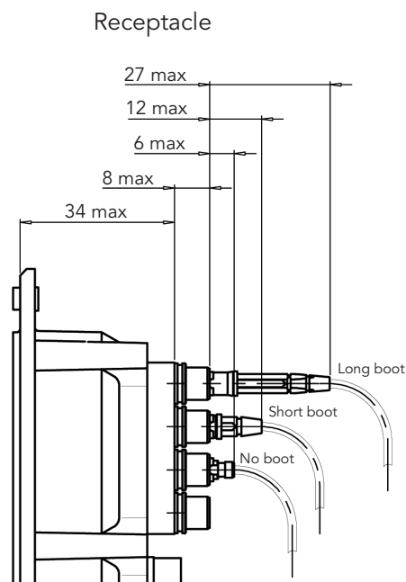
ELIO® contacts in ELIO® AQ adaptor for #8 cavity
