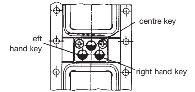
location of polarizing keys (view of engaging face)
