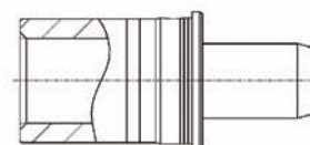
Pin contact
