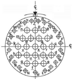
Contact Layout
