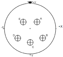
Contact Layout
