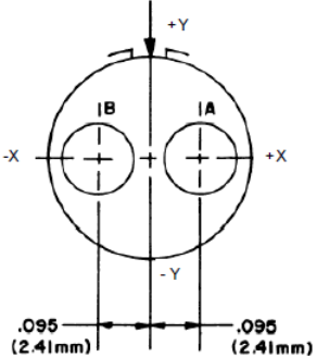
Contact Layout
