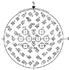
Contact Layout
