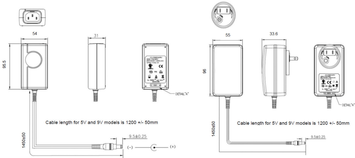
IEC60320 C14 Receptacle, 2.5mm x 5.5mm x 9.5mm Barrel Connector Interchangeable N.A. Blade, 2.5mm x 5.5mm x 9.5mm Barrel Connector
