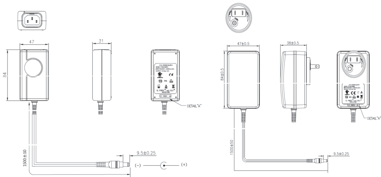
IEC60320C 14 Receptacle, 2.5x5x9.5mm Barrel Connector
