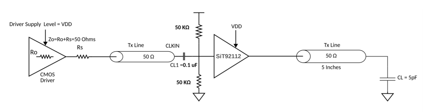
Figure 4. SiT92112 Typical Application Load – AC Coupled Mode
