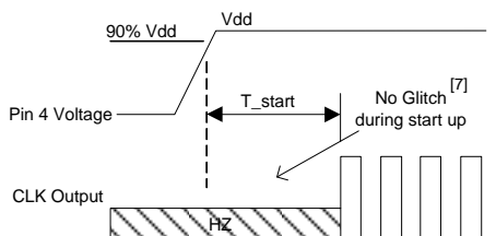
Figure 4. Startup Timing (OE/ST Mode)
