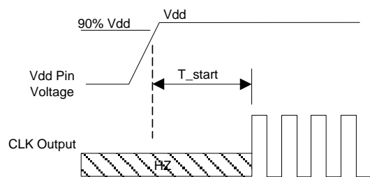
Figure 11. Startup Timing
