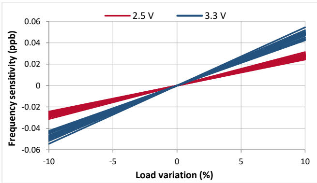
Figure 28. Load sensitivity (±0.1 ppm)
