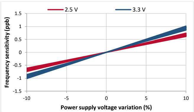
Figure 29. VDD sensitivity (±0.1 ppm)
