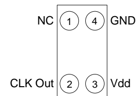
Figure 1. Pin Assignments
