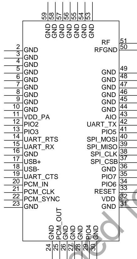
Figure 1: WT41u pin out
