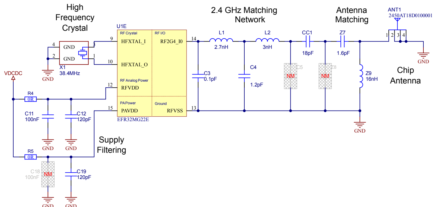
Figure 5.1. Schematic of the RF Section
