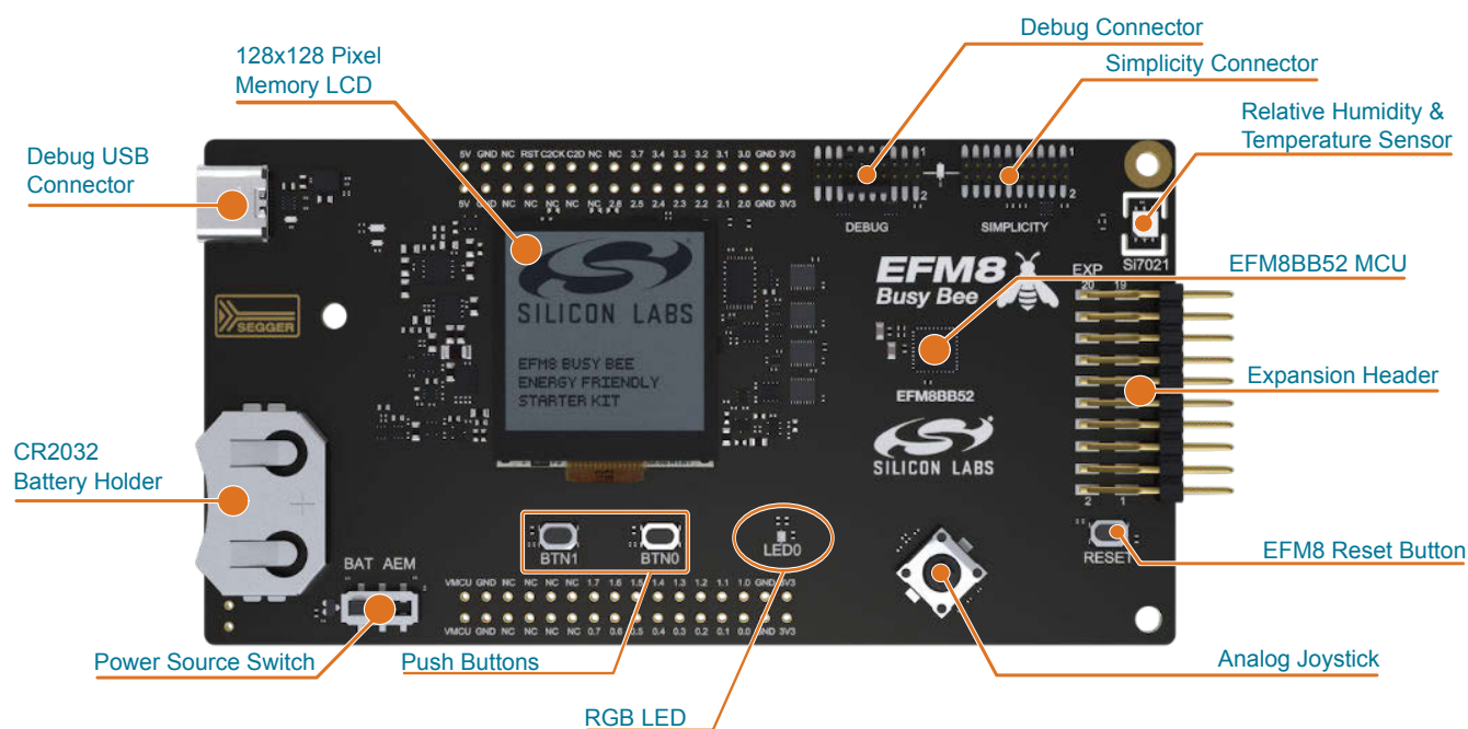
Figure 3.1. BB52 Pro Kit Hardware Layout
