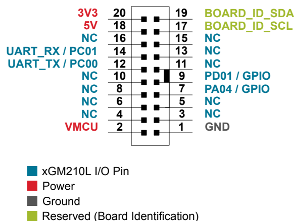
Figure 3.3. EXP Header
