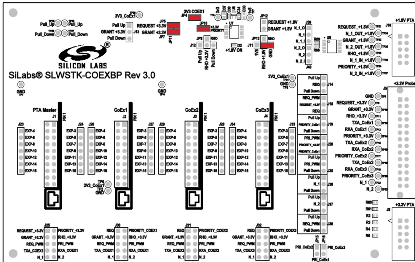
Figure 3.8. PTA Backplane Board J2pers for +1.8V I/O Operation
