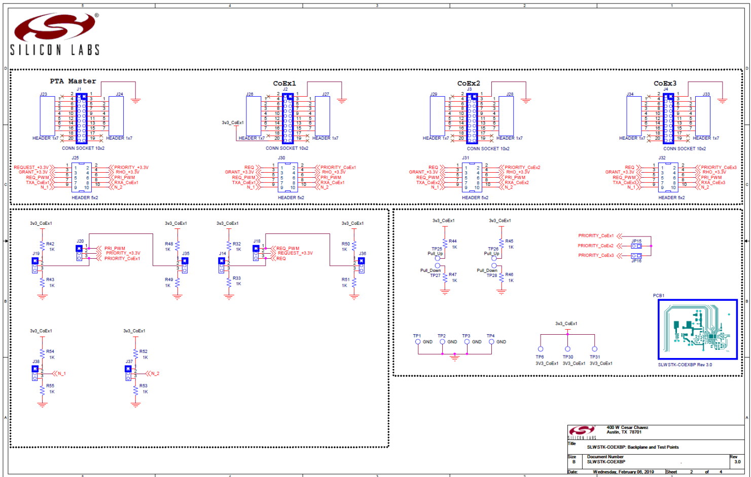
Figure 3.10. SLWSTK-COEXBP Schematic (1/3)
