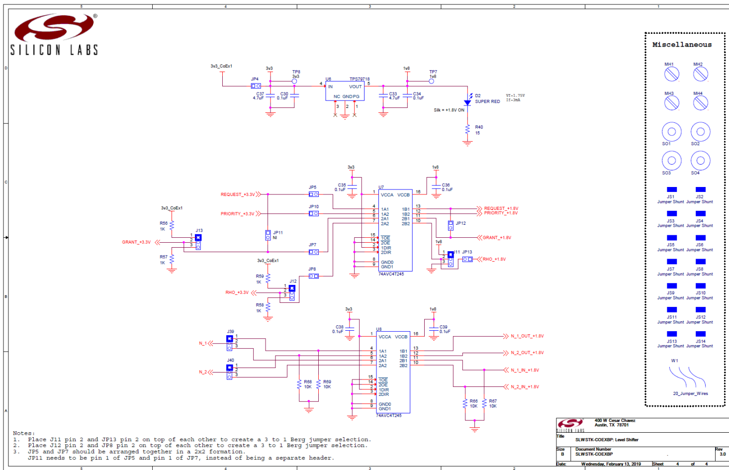
Figure 3.12. SLWSTK-COEXBP Schematic (3/3)
