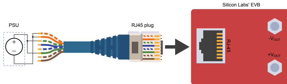
Figure 2.2. Midspan Connection using Laboratory Power Supply
