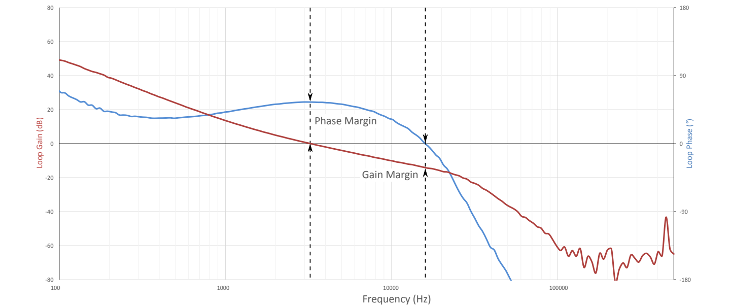
Figure 5.1. Si3404ISOFB-EVB Measured Loop-Gain and Phase Shift
