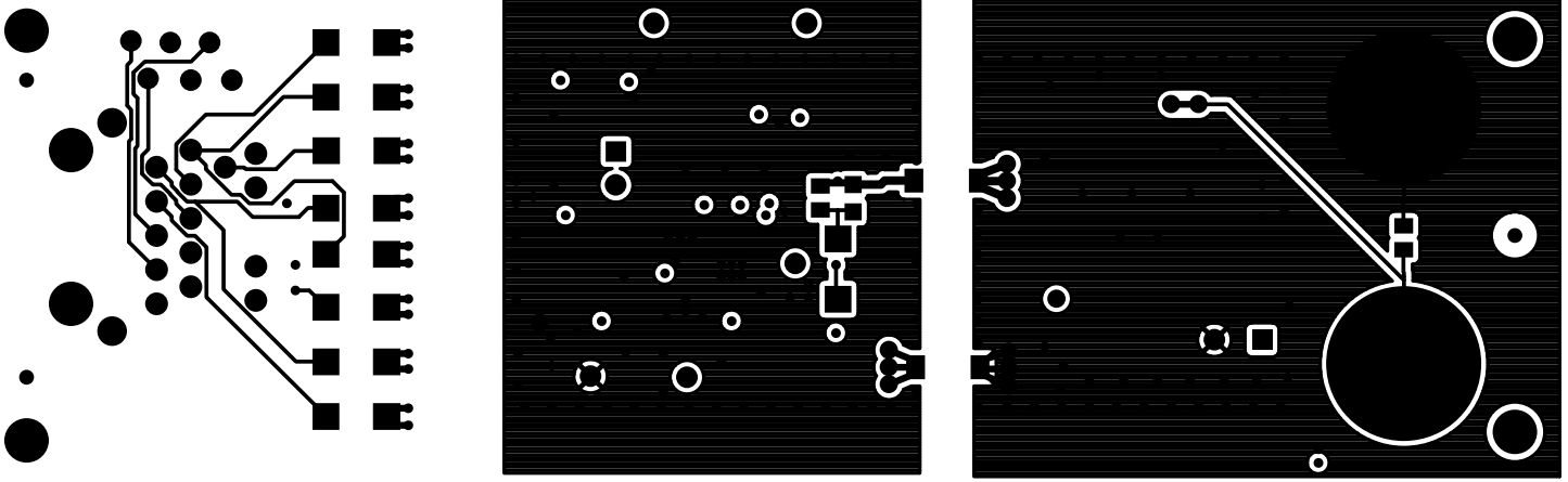
Figure 16.5. Bottom Layer
