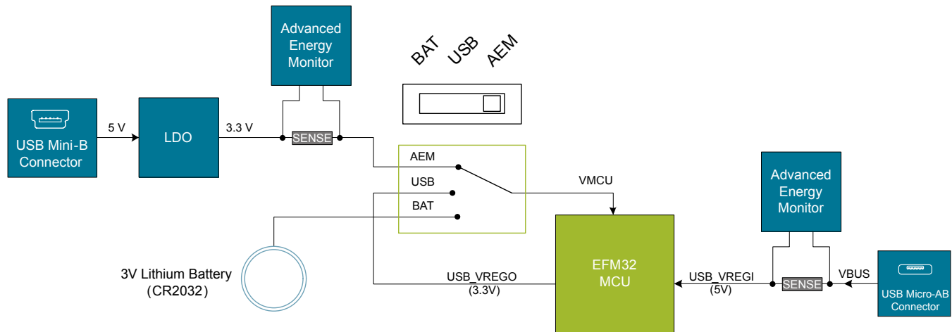
Figure 5.1. Power Switch
