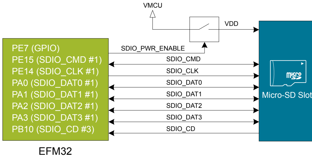
Figure 6.10. Micro-SD Slot
