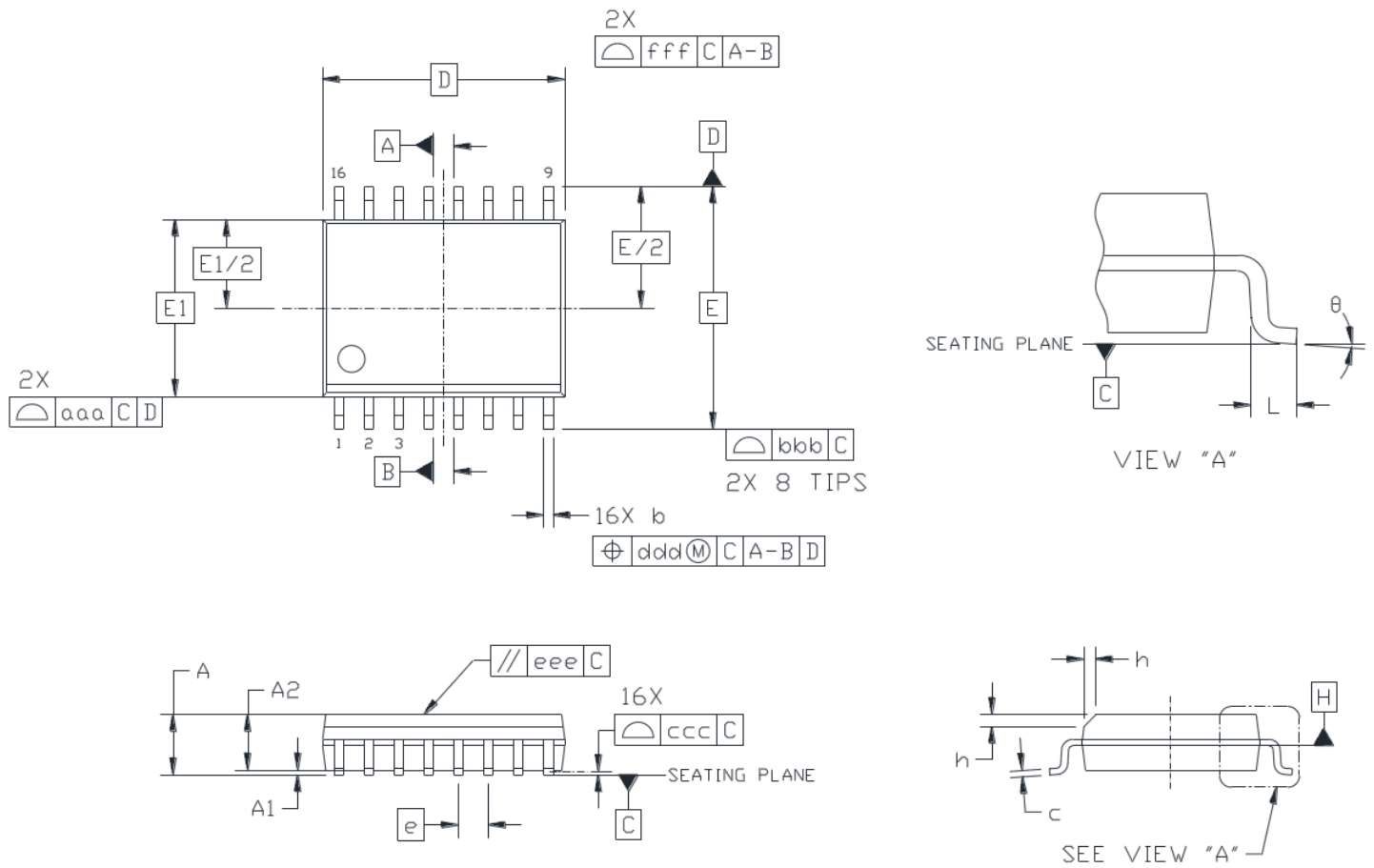
Figure 8.1. WB SOIC-16
