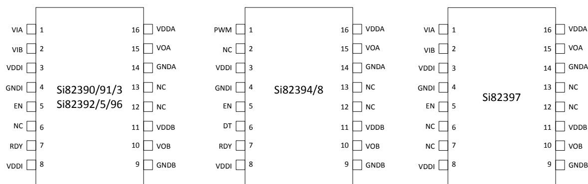
Figure 6.1. Si8239x SOIC-16 1
