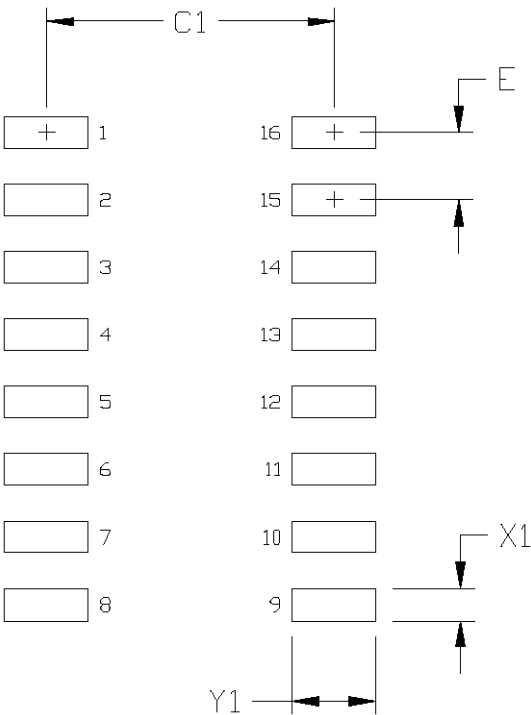
Figure 12.1. 16-Pin Narrow Body SOIC PCB Land Pattern
