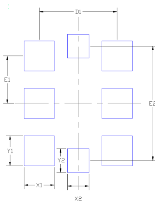
Figure 7.3. Si549 (2.5x3.2 mm) PCB Land Pattern
