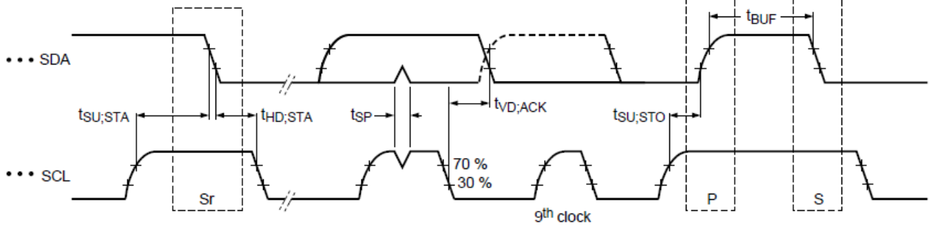
Figure 6.1. I 2 C Serial Port Timing Standard and Fast Modes
