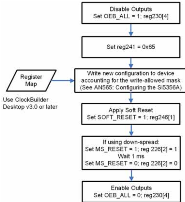
Figure 5. I 2 C Programming Procedure
