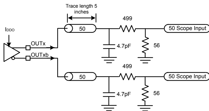
LVCMOS Output Test Configuration
