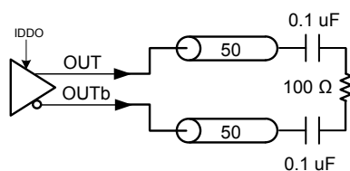
Differential Output Test Configuration
