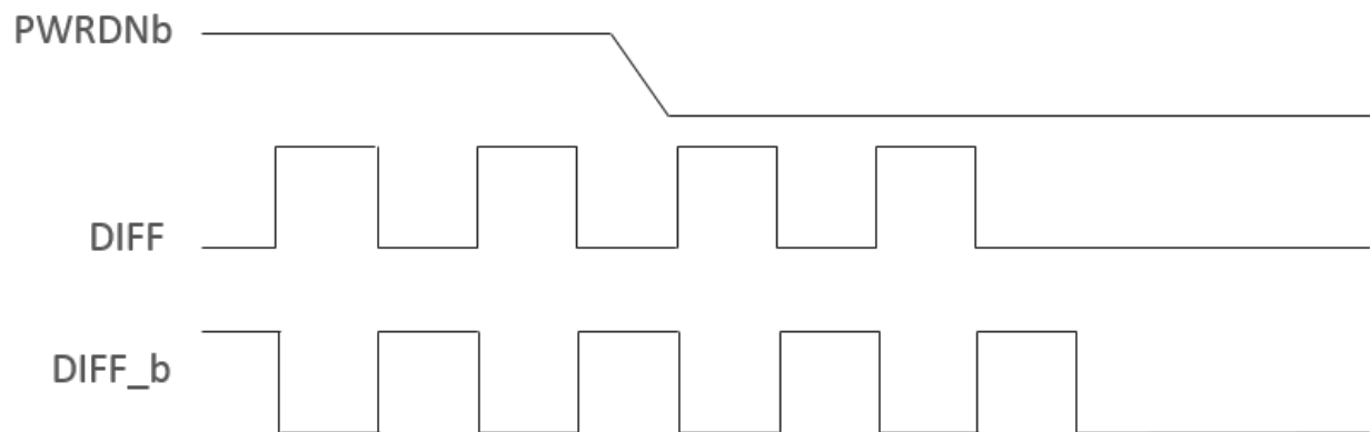
Figure 5.5. PWRDNb Assertion
