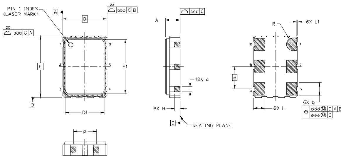
Figure 9. Si514 Outline Diagram
