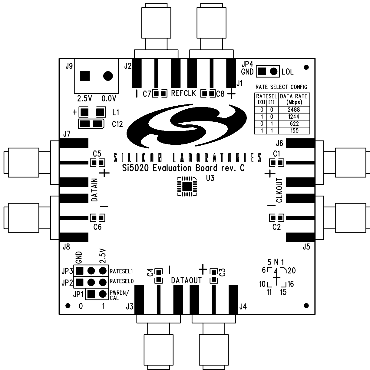
Figure 4. Si5020 Silkscreen
