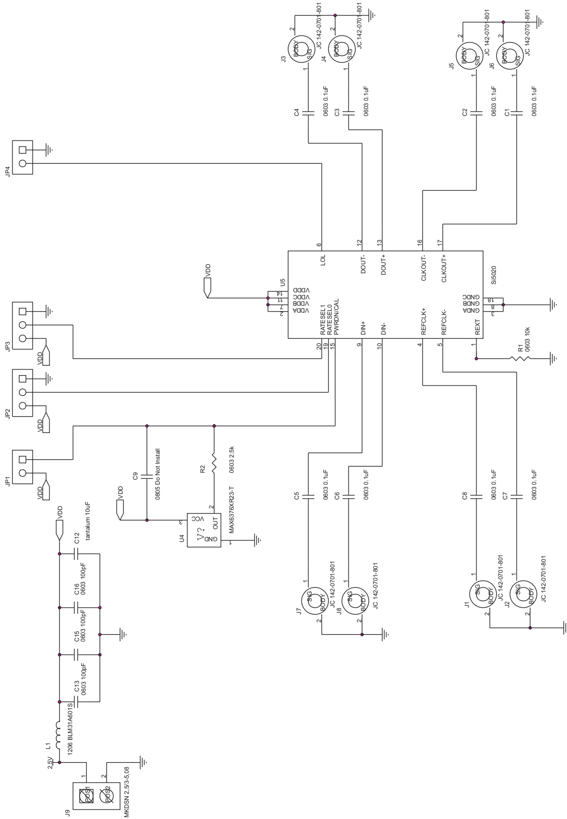
Figure 3. Si5020 Schematic
