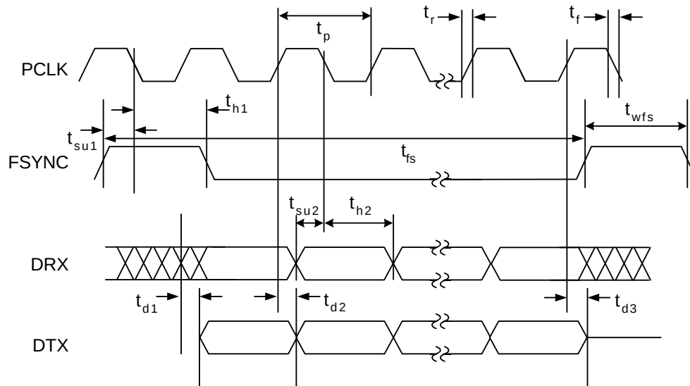
Figure 3. PCM Highway Interface Timing Diagram
