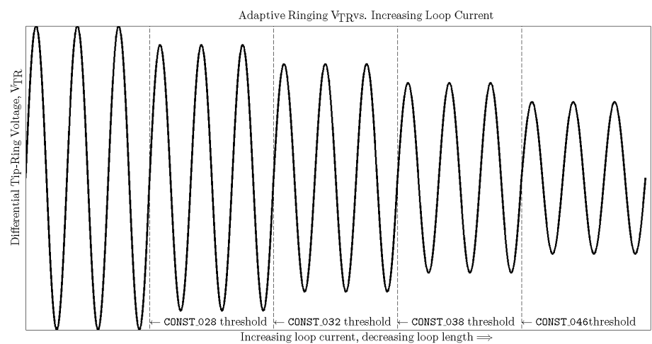
Figure 23. Adaptive Ringing
