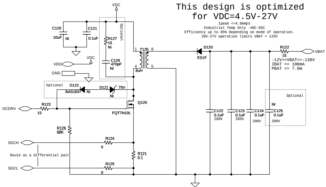
Figure 12. Flyback Tracking DC DC2
